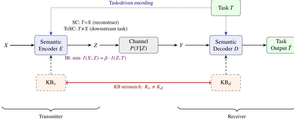
Fig. 5. Consolidated ToSC system model with IB notation. The semantic encoder E , conditioned on source knowledge base KB_s , compresses source X into representation Z . The decoder D , conditioned on KB_d , produces the task output \hat{T} . The IB objective governs the compression–task-relevance trade-off: SC corresponds to T=X (full reconstruction), while ToSC targets a downstream task T \neq X , discarding task-irrelevant information. The red link highlights that KB mismatch ( K_s \neq K_d ) introduces semantic noise independent of channel quality.
