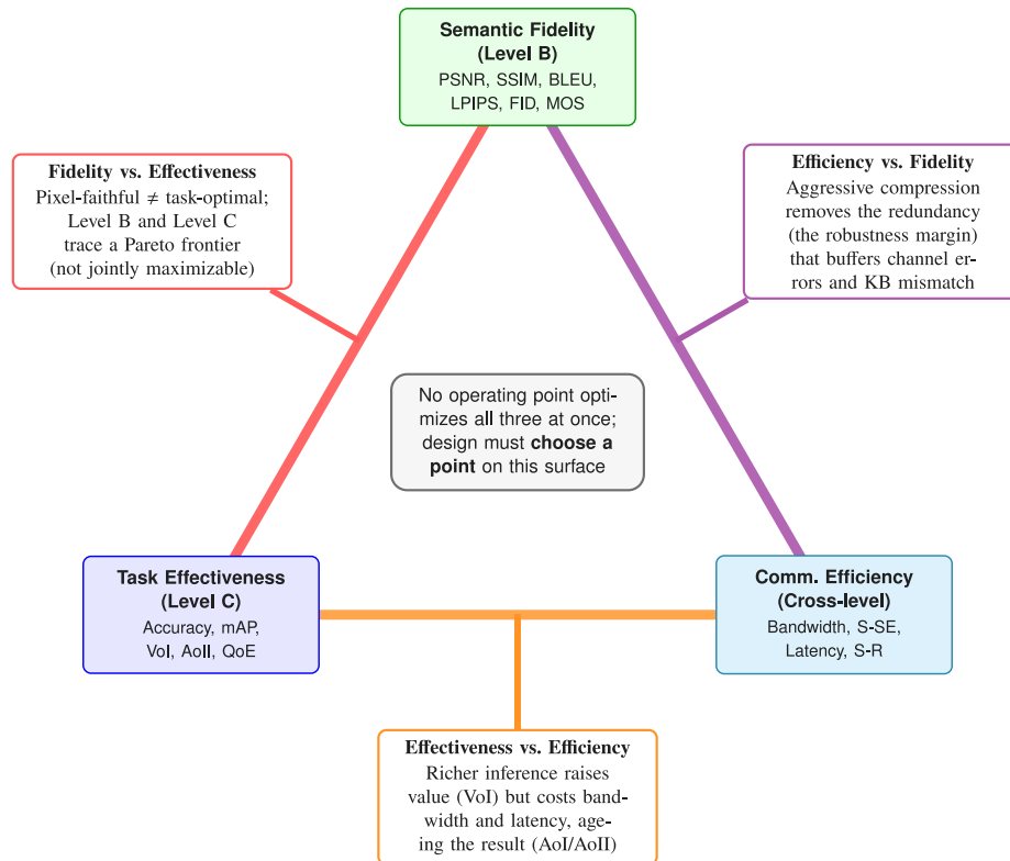
Fig. 6. Metric conflict and trade-off map for SC/ToSC evaluation. The three vertices are the primary metric families: semantic fidelity (Level B), task effectiveness (Level C), and communication efficiency (cross-level). Each edge denotes a pairwise conflict with its governing mechanism: fidelity vs. effectiveness (the Level B and Level C objectives trace a Pareto frontier and cannot be jointly maximized), effectiveness vs. efficiency (richer inference raises value-of-information but costs bandwidth and increases age-of-information), and efficiency vs. fidelity (aggressive compression removes the redundancy, i.e. the robustness margin, that buffers channel errors and knowledge-base mismatch). As the central node states, no single operating point optimizes all three simultaneously, so system design reduces to selecting a justified point on this surface.
