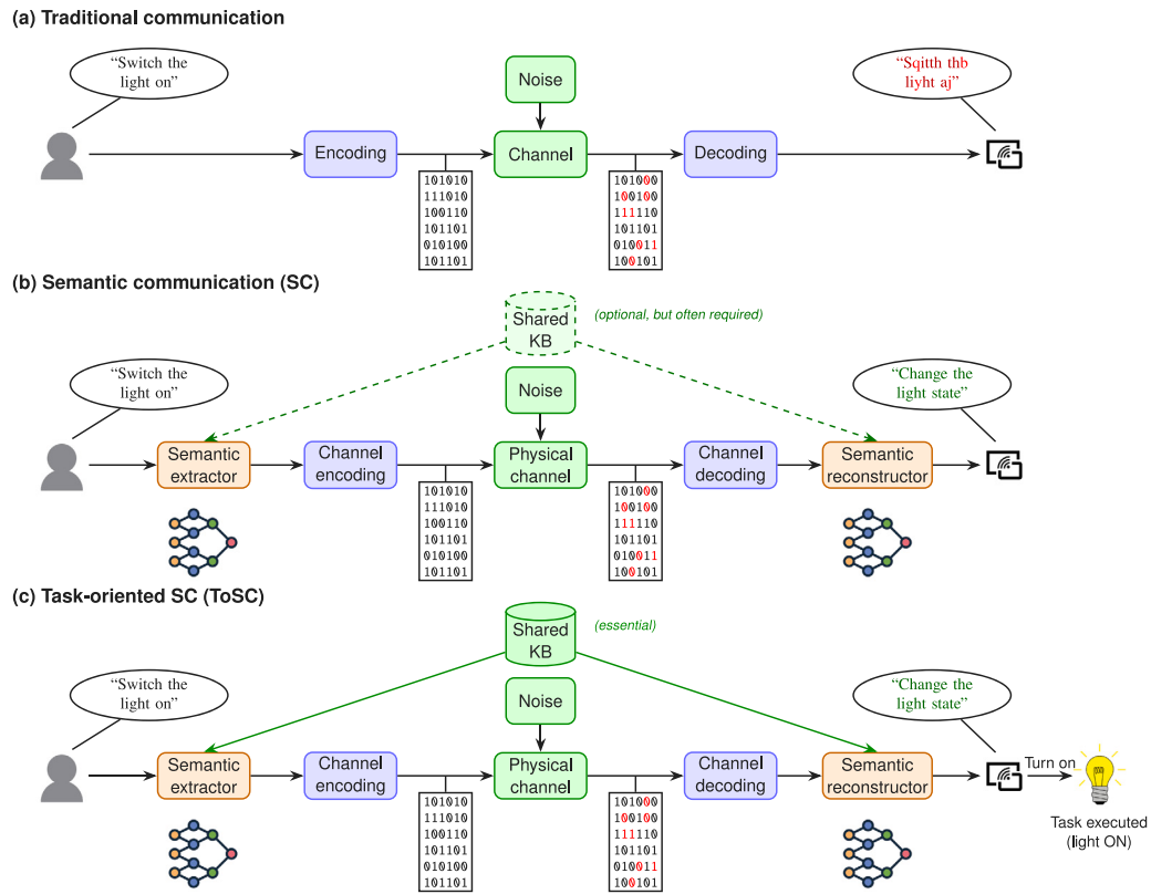
Fig. 4. Comparative study of traditional models, SC systems, and ToSC systems: workflow of (a) traditional communication, (b) SC, and (c) ToSC. In (a) every bit must be recovered, so channel errors corrupt the delivered message. In (b) the semantic extractor and reconstructor exchange a learned semantic representation, and the receiving system recovers the intended meaning despite bit errors. In (c) the ToSC pipeline conveys only the semantics the receiving system needs to execute the task (switching the light on), rather than the full semantic content. A shared knowledge base supports semantic interpretation in both paradigms; as marked in the figure, it is optional, but often required, for general SC (dashed) and essential for ToSC's task relevance and interpretation (solid; Table 2).
