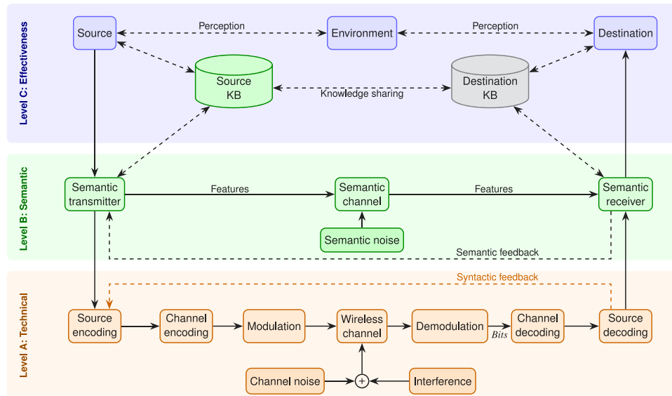
Fig. 2. Weaver’s three levels of communication (Level A: Technical, Level B: Semantic, and Level C: Effectiveness). The mapping of these levels to the performance metrics is discussed in Section 4; ToSC primarily targets Level C.
